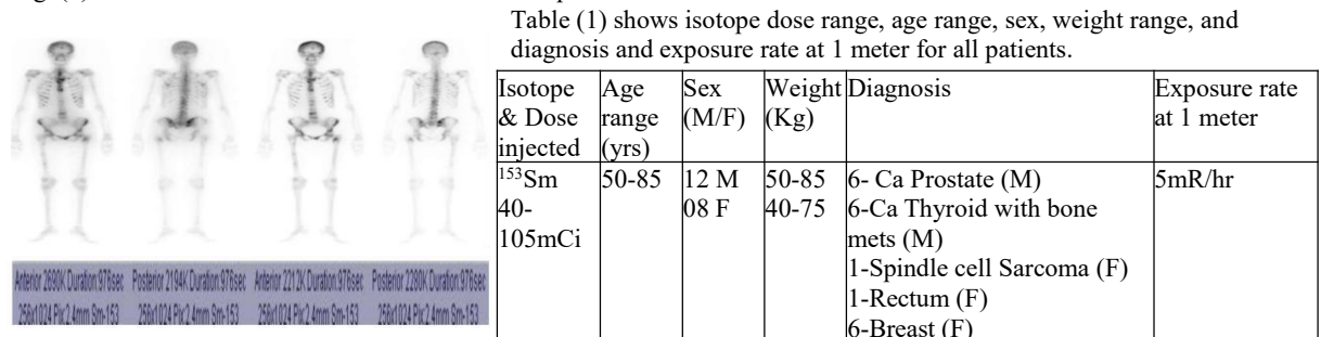
Fig. (1) shows WB Scan of 153 Sm confirmation of uptake in metastatic areas.
