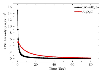
Fig. 1. CW-OSL decay curve of \text{LiCaAlF}_6 : Eu and \text{Al}_2\text{O}_3 :C (BARC) after irradiation with 500mGy beta dose
